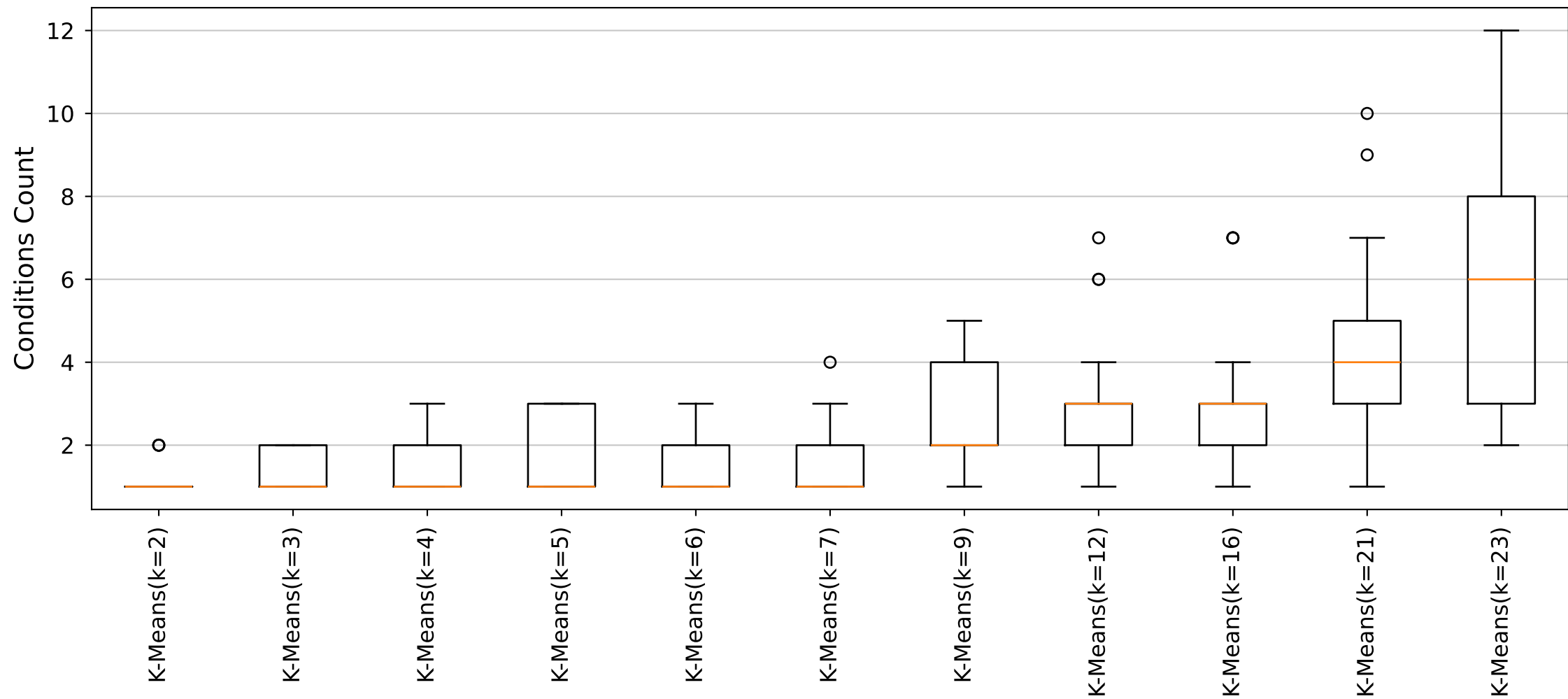
YARA Rules Conditions Count Distribution (Cluster5_Size23 dataset)
